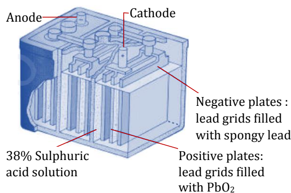
Fig: The Lead storage battery
