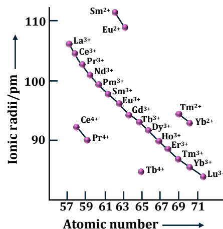
Trends in ionic radii of lanthanides
