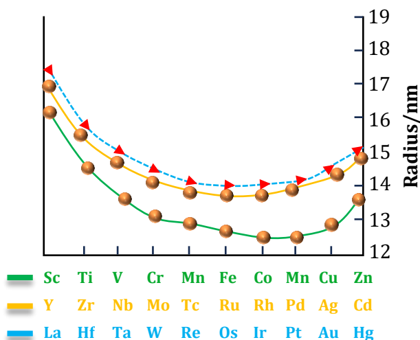
Trends in atomic radii of transition elements
