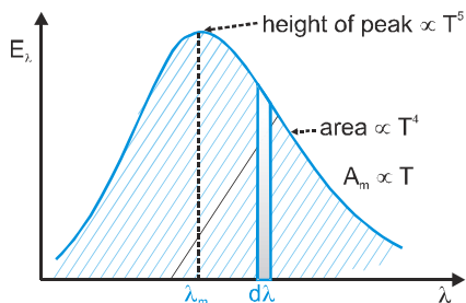
spectral energy distribution curve ( E_\lambda - \lambda )
